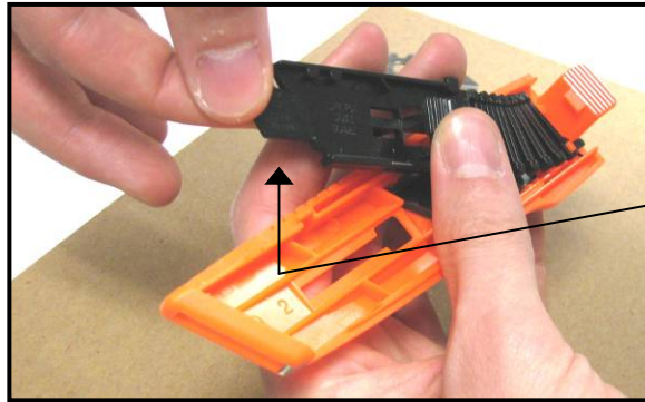
Bend the tab on the front of the slider back and forth several times.
